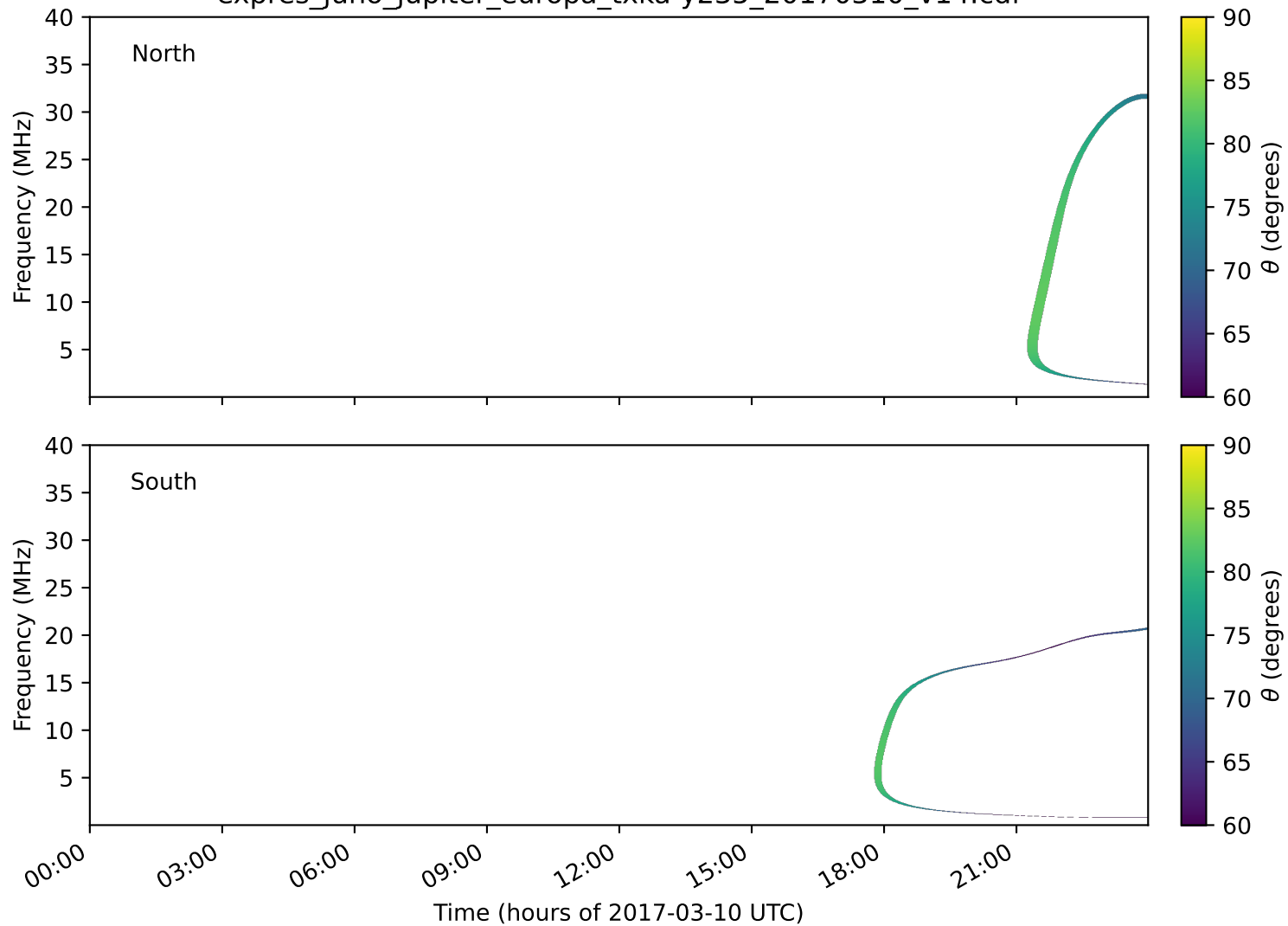
expres_juno_jupiter_europa_txka-y235_20170310_v14.cdf
