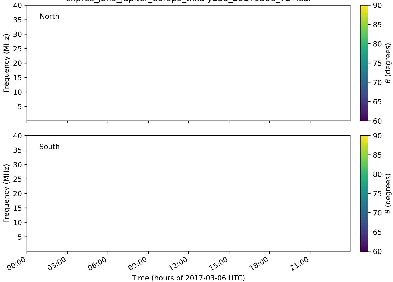
expres_juno_jupiter_europa_txka-y235_20170306_v14.cdf
