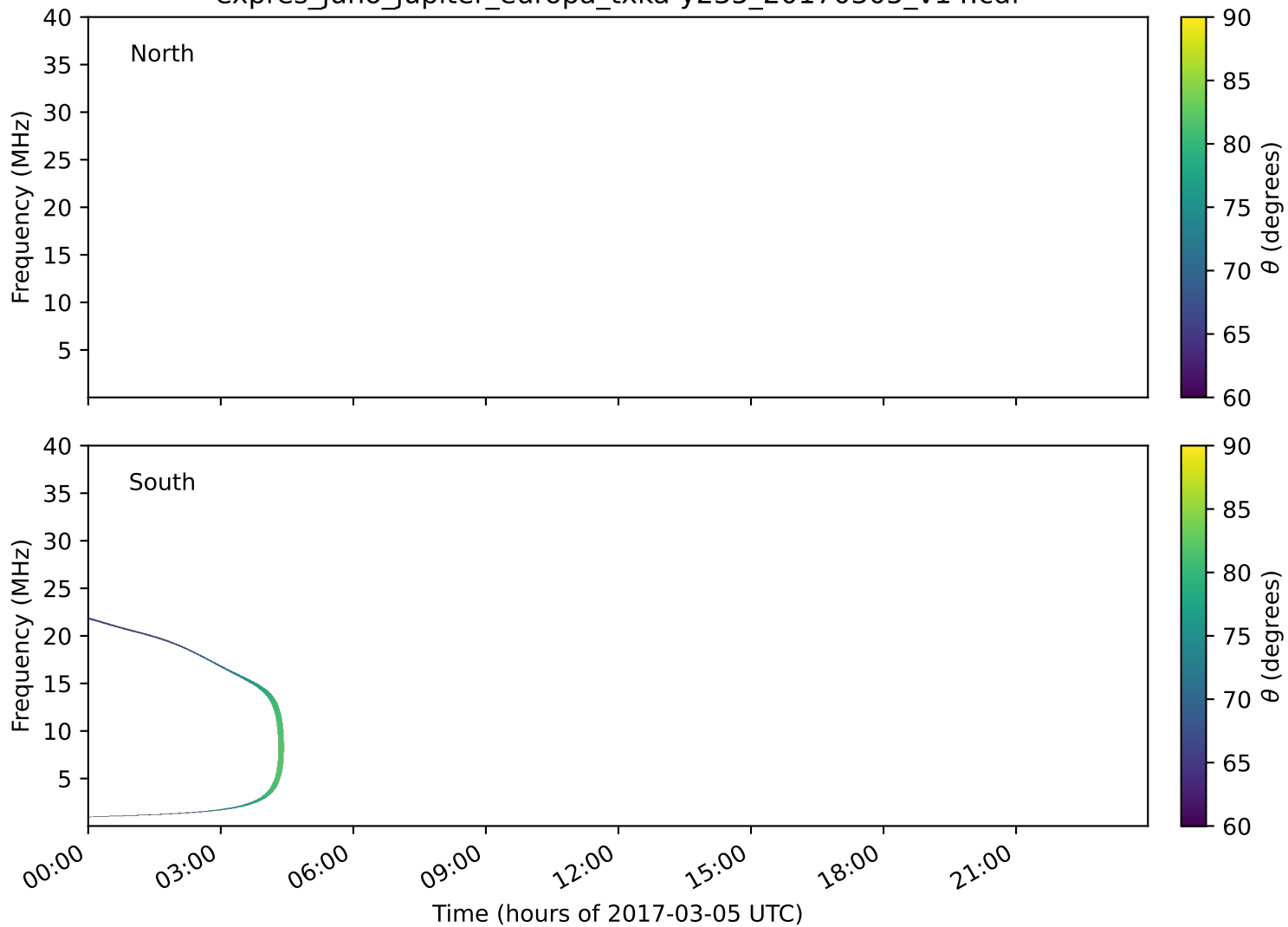
expres_juno_jupiter_europa_txka-y235_20170305_v14.cdf
