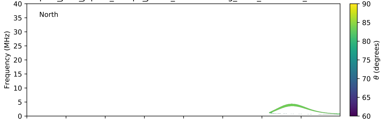
expres_juno_jupiter_europa_jrm09_lossc-wid1deg_3kev_20170328_v01.cdf
