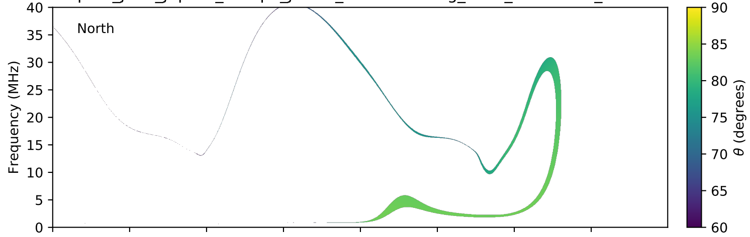
expres_juno_jupiter_europa_jrm09_lossc-wid1deg_3kev_20170326_v01.cdf
