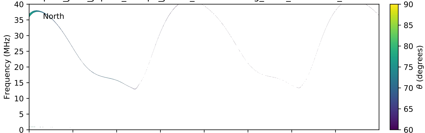
expres_juno_jupiter_europa_jrm09_lossc-wid1deg_3kev_20170325_v01.cdf
