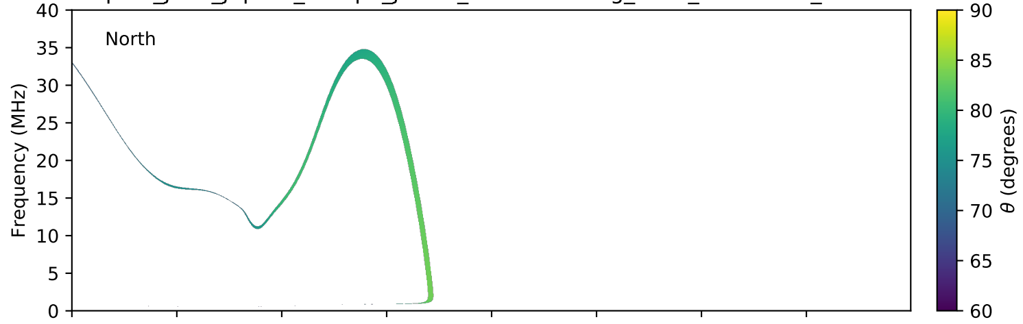
expres_juno_jupiter_europa_jrm09_lossc-wid1deg_3kev_20170319_v01.cdf
