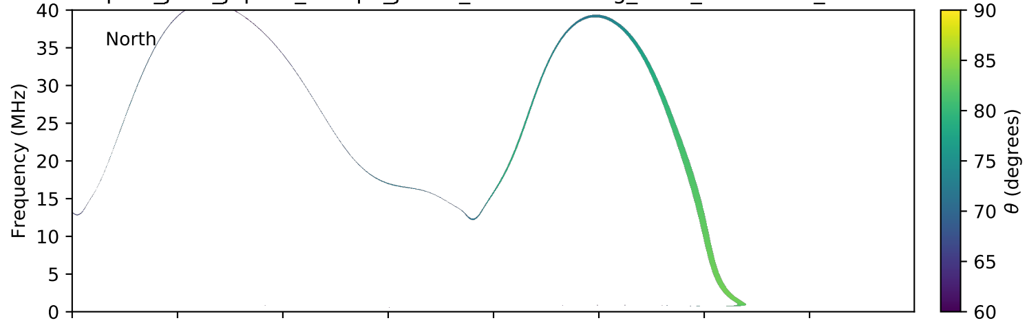
expres_juno_jupiter_europa_jrm09_lossc-wid1deg_3kev_20170315_v01.cdf
