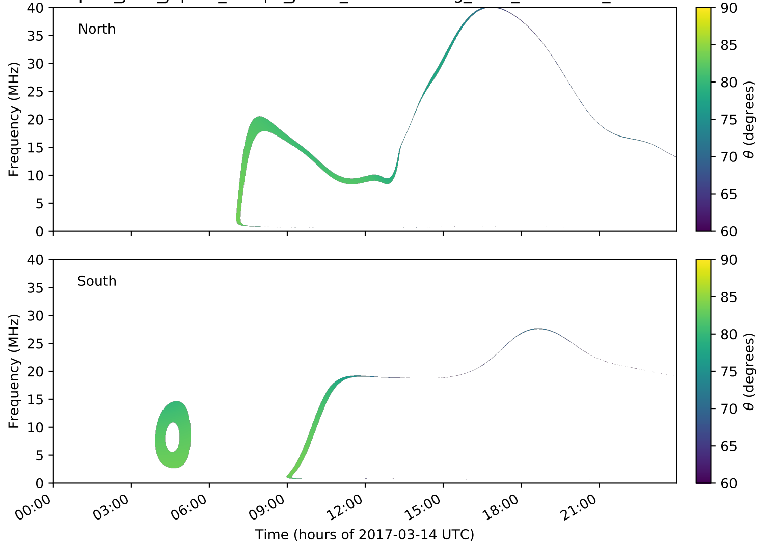
expres_juno_jupiter_europa_jrm09_lossc-wid1deg_3kev_20170314_v01.cdf
