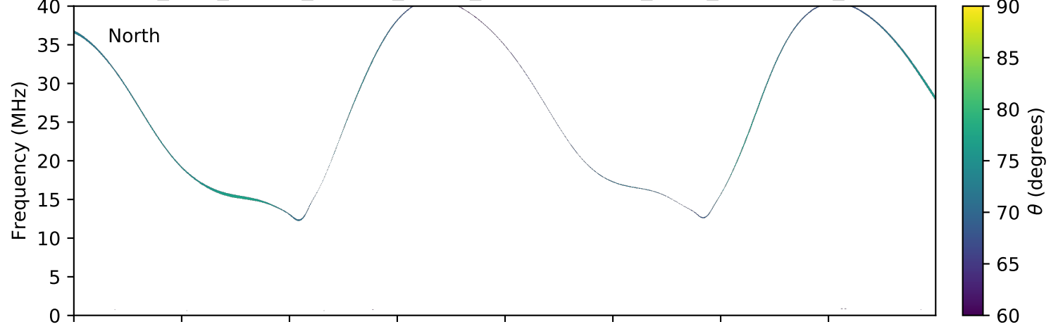
expres_juno_jupiter_europa_jrm09_lossc-wid1deg_3kev_20170311_v01.cdf
