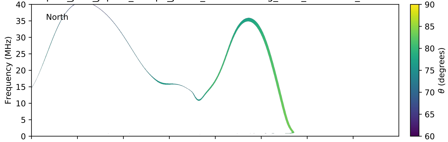
expres_juno_jupiter_europa_jrm09_lossc-wid1deg_3kev_20170308_v01.cdf
