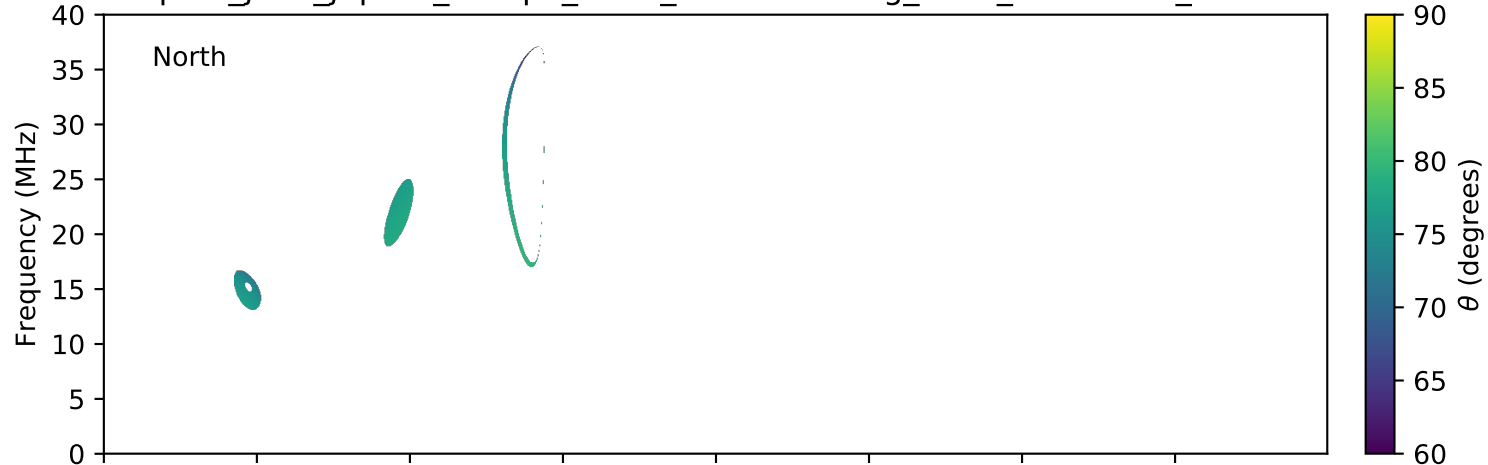
expres_juno_jupiter_europa_isaac_lossc-wid1deg_5kev_20170327_v01.cdf
