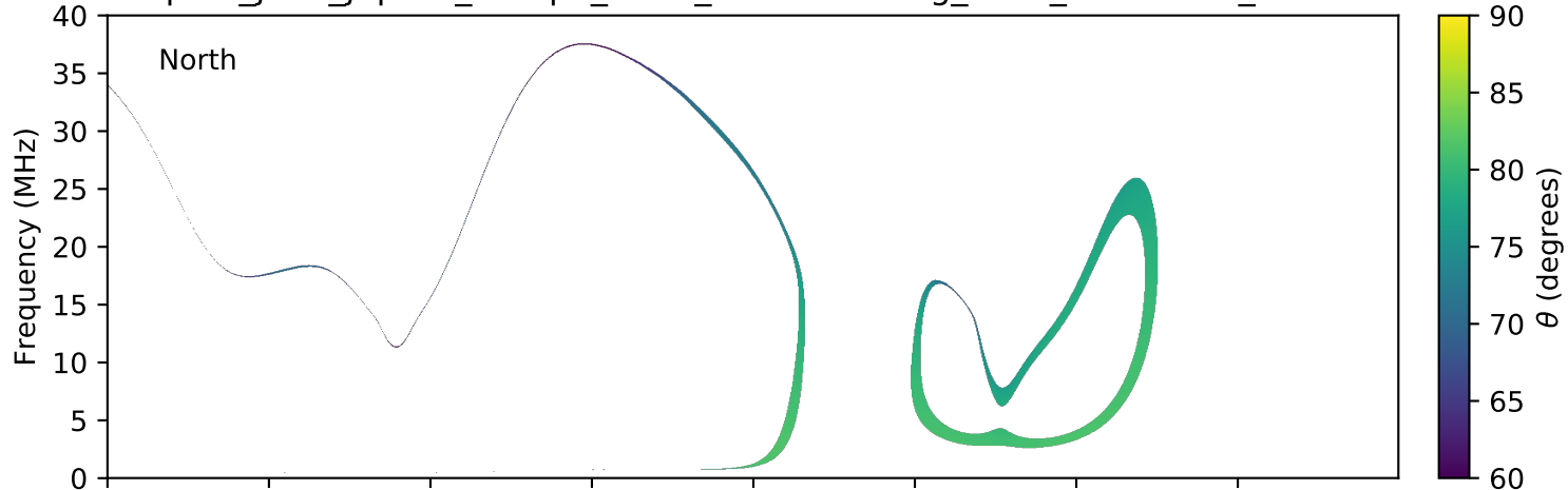
expres_juno_jupiter_europa_isaac_lossc-wid1deg_5kev_20170326_v01.cdf
