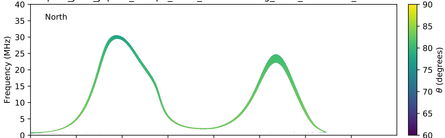
expres_juno_jupiter_europa_isaac_lossc-wid1deg_3kev_20170329_v01.cdf
