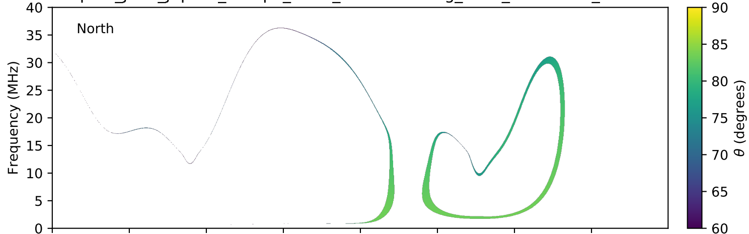
expres_juno_jupiter_europa_isaac_lossc-wid1deg_3kev_20170326_v01.cdf
