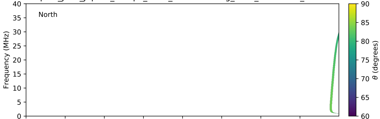
expres_juno_jupiter_europa_isaac_lossc-wid1deg_3kev_20170324_v01.cdf
