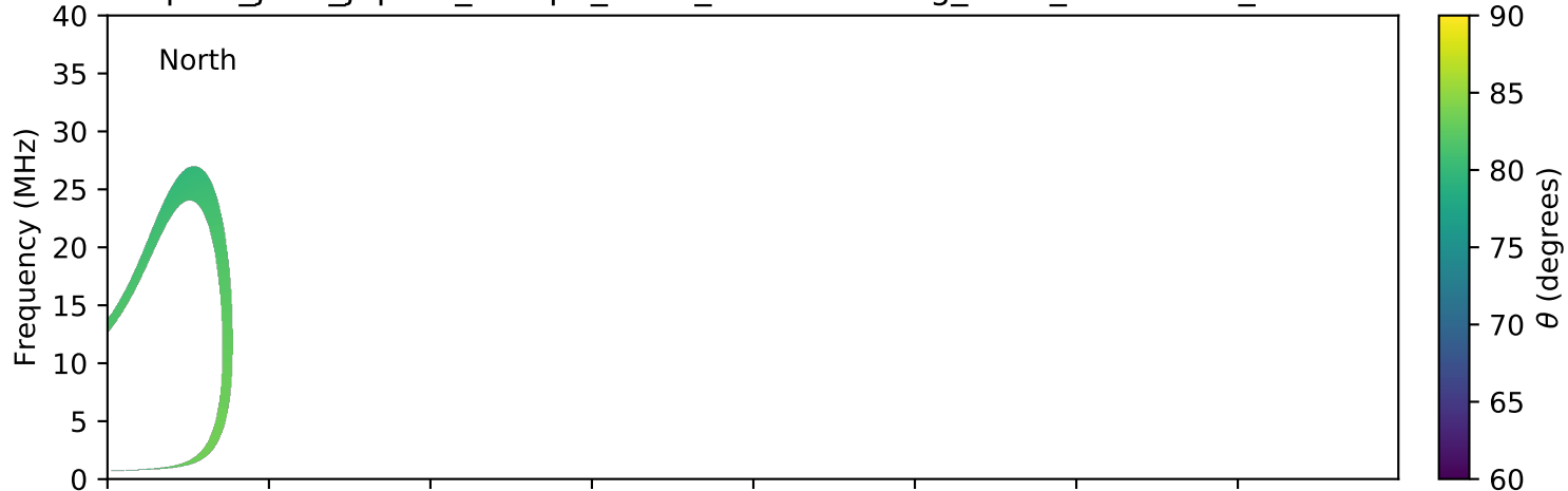
expres_juno_jupiter_europa_isaac_lossc-wid1deg_3kev_20170323_v01.cdf
