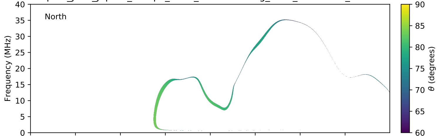
expres_juno_jupiter_europa_isaac_lossc-wid1deg_3kev_20170321_v01.cdf
