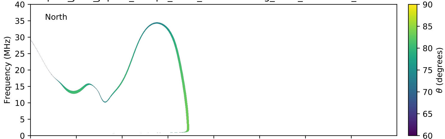
expres_juno_jupiter_europa_isaac_lossc-wid1deg_3kev_20170319_v01.cdf
