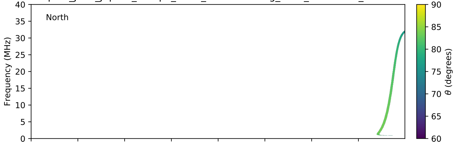
expres_juno_jupiter_europa_isaac_lossc-wid1deg_3kev_20170317_v01.cdf
