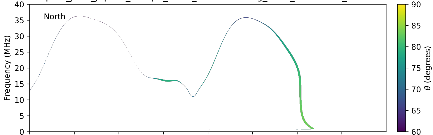
expres_juno_jupiter_europa_isaac_lossc-wid1deg_3kev_20170315_v01.cdf
