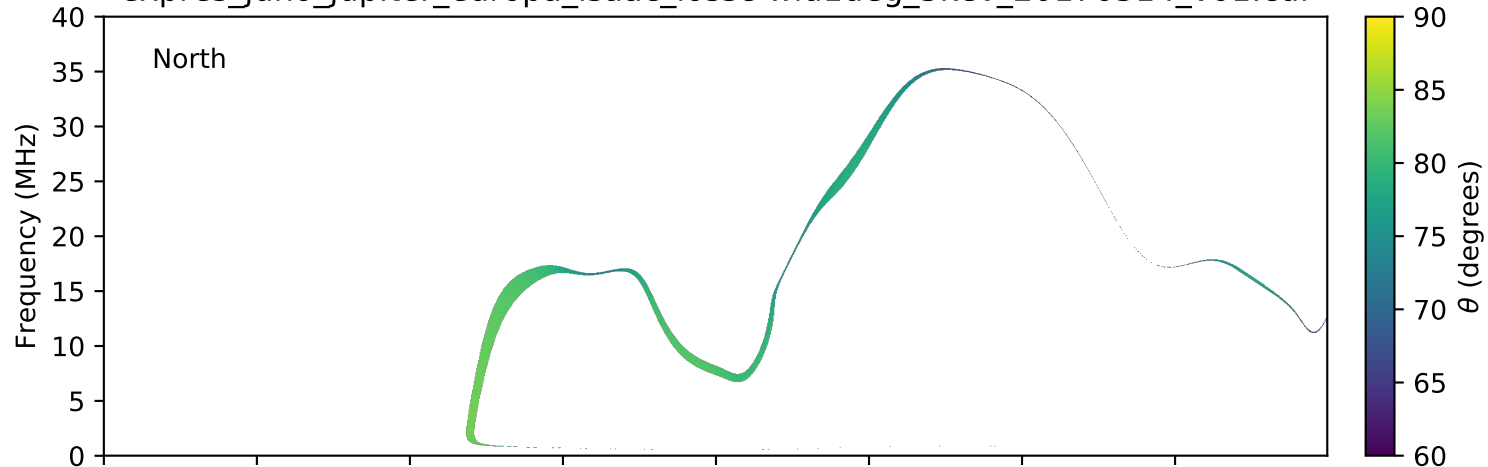
expres_juno_jupiter_europa_isaac_lossc-wid1deg_3kev_20170314_v01.cdf
