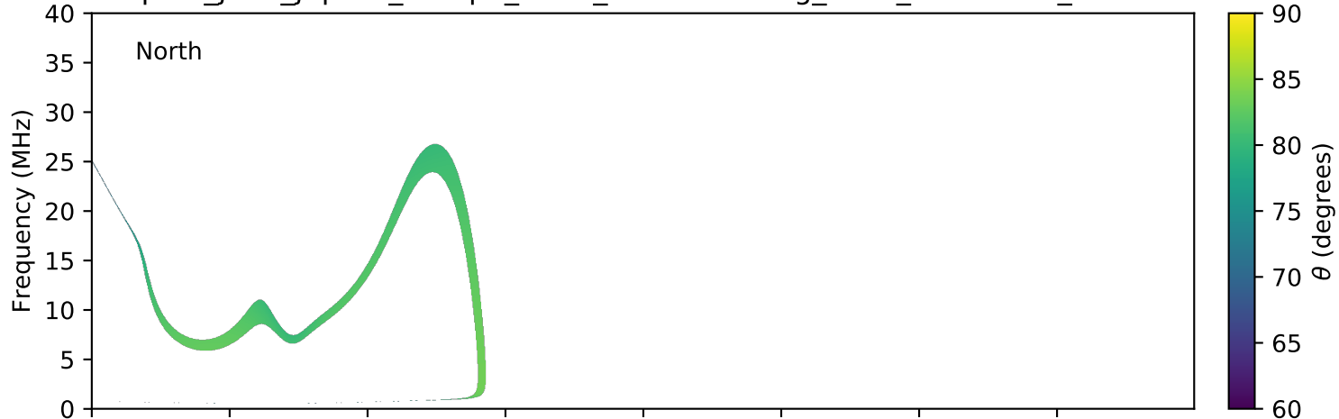
expres_juno_jupiter_europa_isaac_lossc-wid1deg_3kev_20170312_v01.cdf
