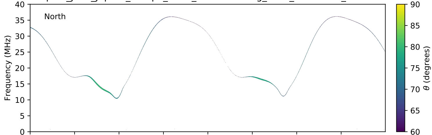
expres_juno_jupiter_europa_isaac_lossc-wid1deg_3kev_20170311_v01.cdf
