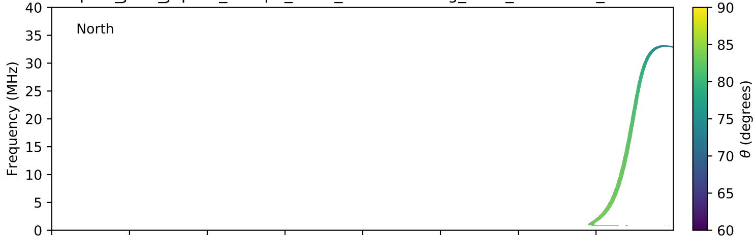
expres_juno_jupiter_europa_isaac_lossc-wid1deg_3kev_20170310_v01.cdf
