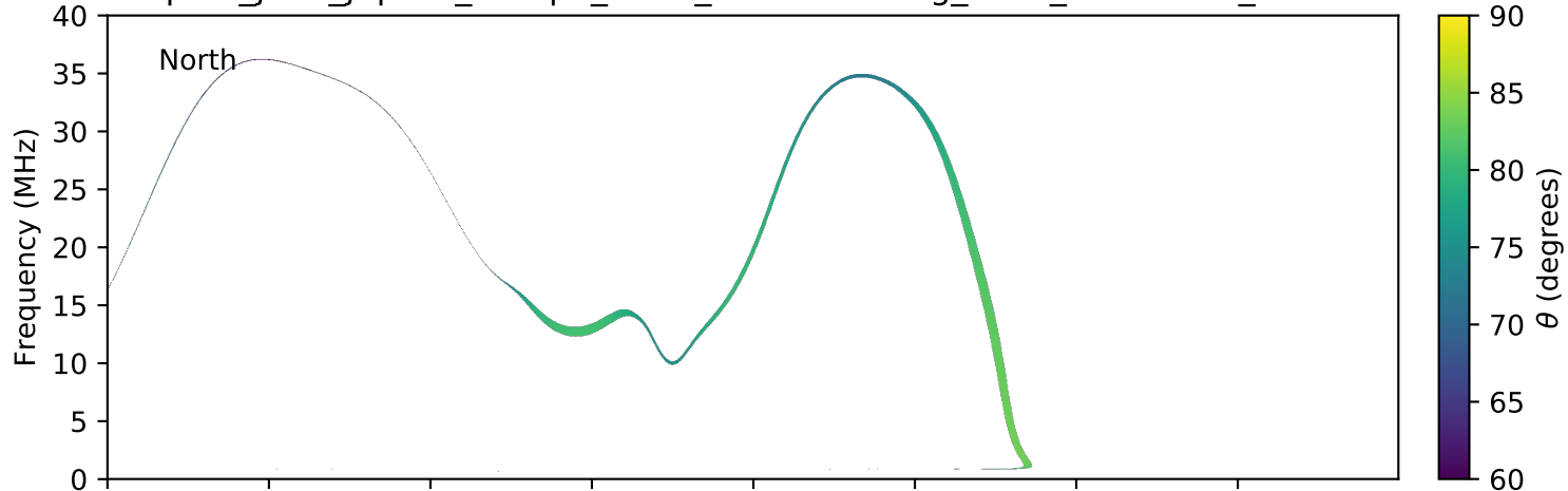
expres_juno_jupiter_europa_isaac_lossc-wid1deg_3kev_20170308_v01.cdf
