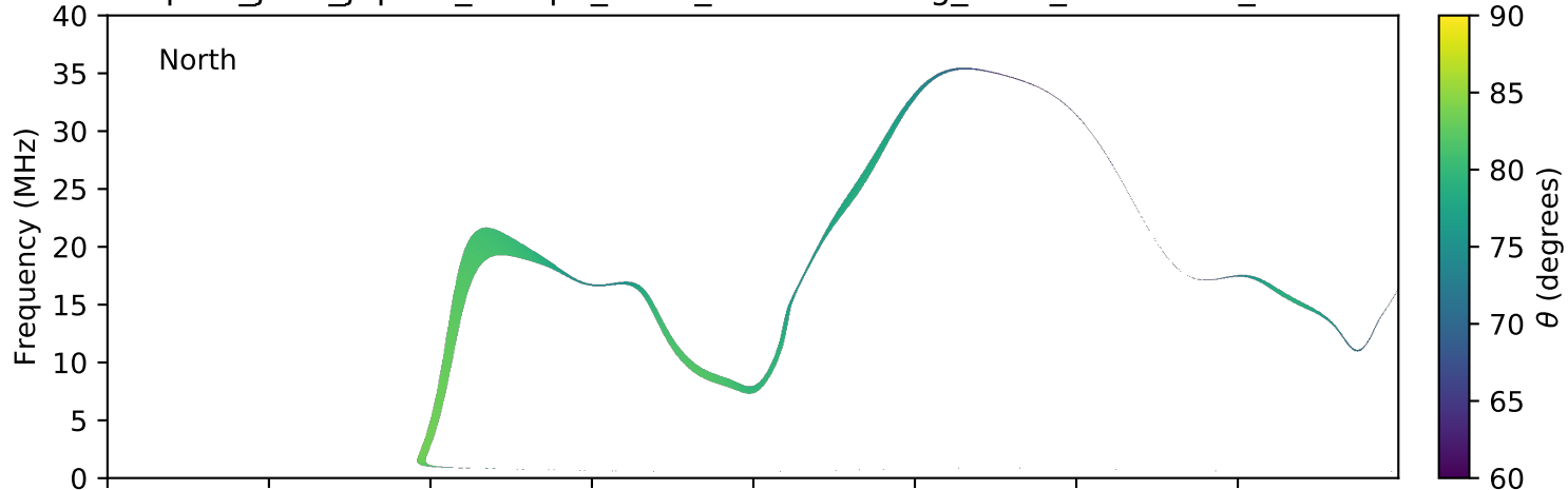
expres_juno_jupiter_europa_isaac_lossc-wid1deg_3kev_20170307_v01.cdf
