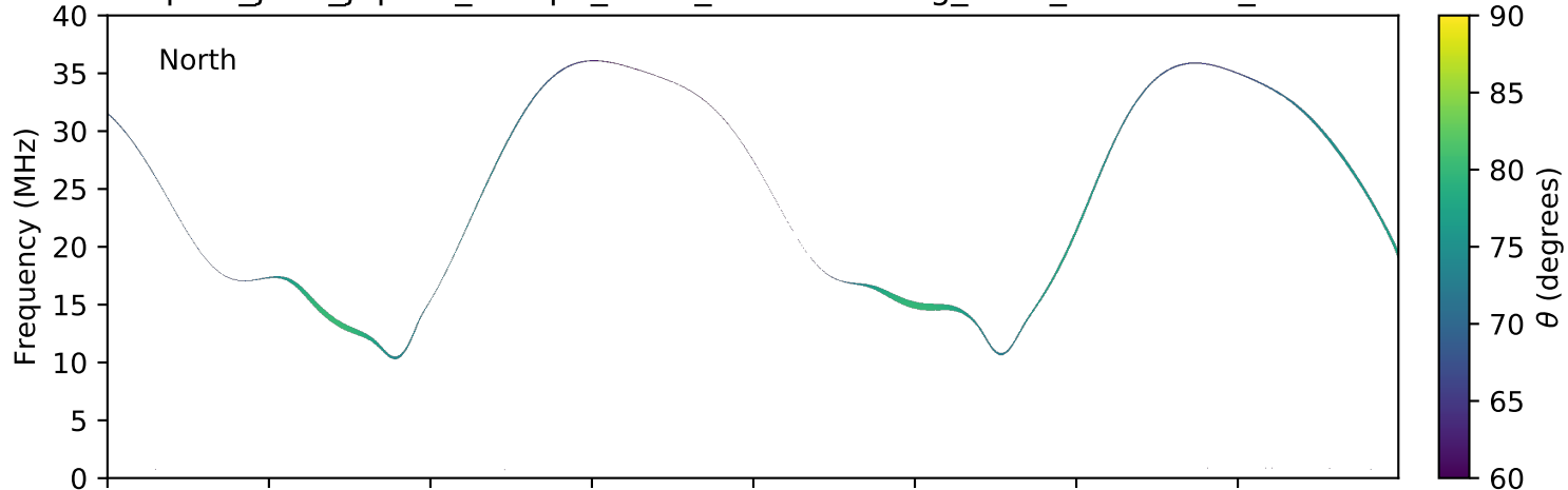
expres_juno_jupiter_europa_isaac_lossc-wid1deg_3kev_20170304_v01.cdf
