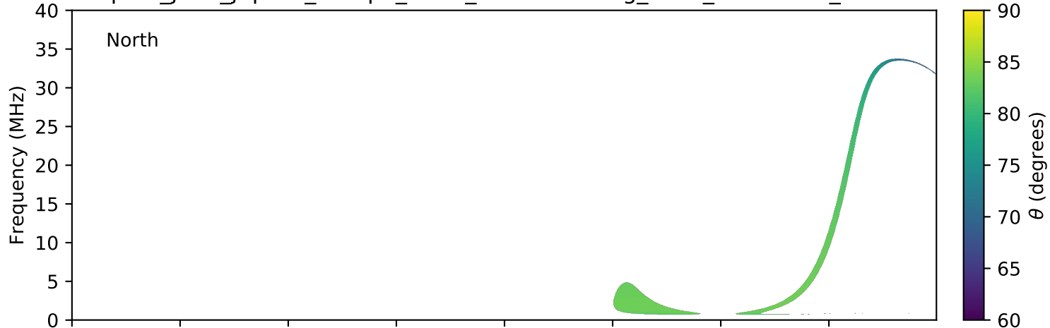
expres_juno_jupiter_europa_isaac_lossc-wid1deg_3kev_20170303_v01.cdf
