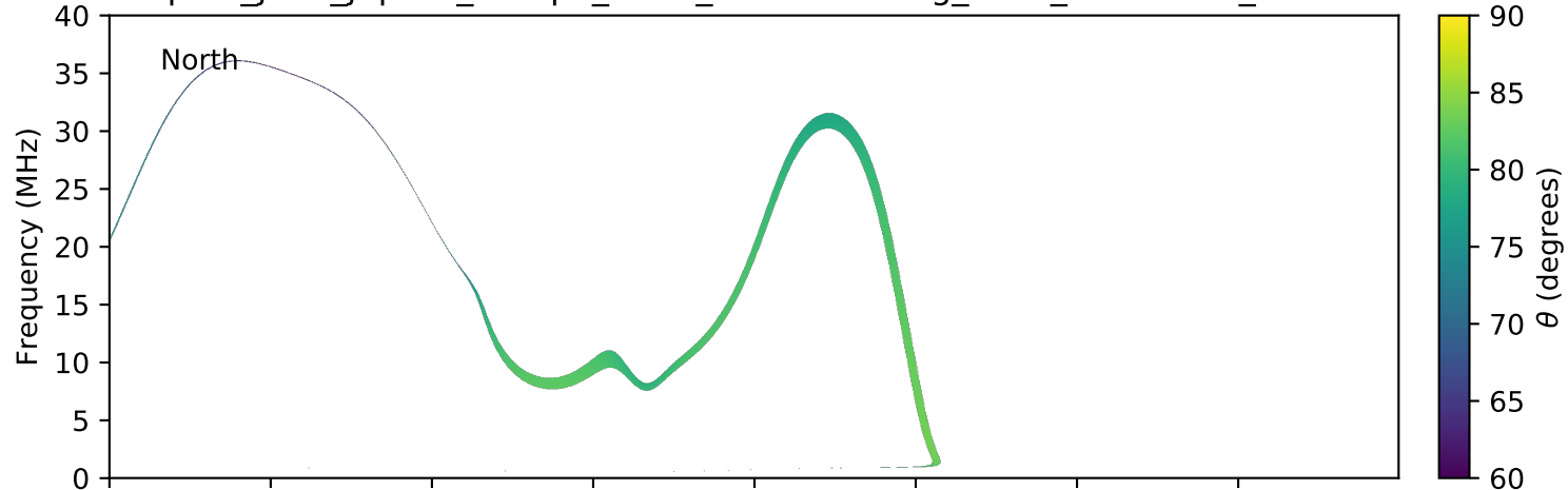
expres_juno_jupiter_europa_isaac_lossc-wid1deg_3kev_20170301_v01.cdf
