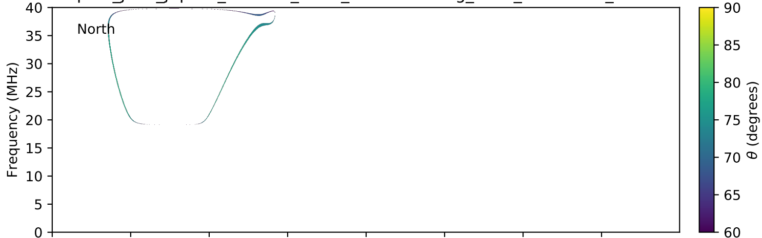
expres_juno_jupiter_218d-0r_isaac_lossc-wid1deg_9kev_20170327_v01.cdf
