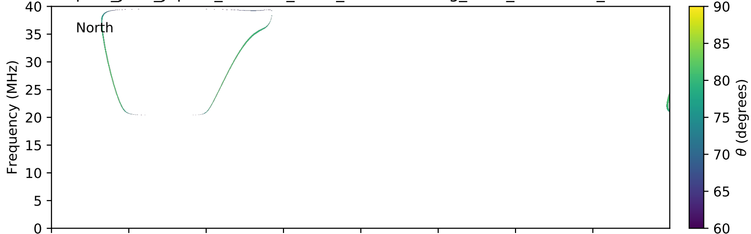
expres_juno_jupiter_218d-0r_isaac_lossc-wid1deg_5kev_20170327_v01.cdf
