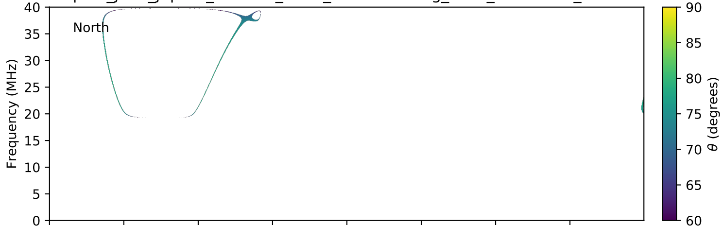
expres_juno_jupiter_217d-0r_isaac_lossc-wid1deg_9kev_20170327_v01.cdf
