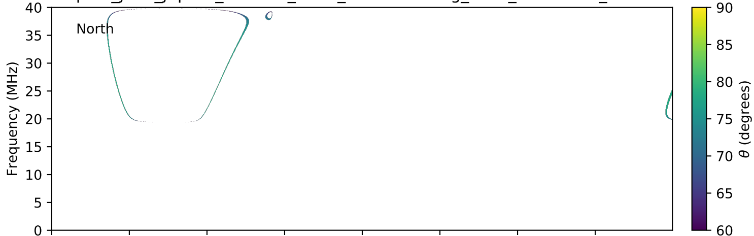
expres_juno_jupiter_215d-0r_isaac_lossc-wid1deg_9kev_20170327_v01.cdf
