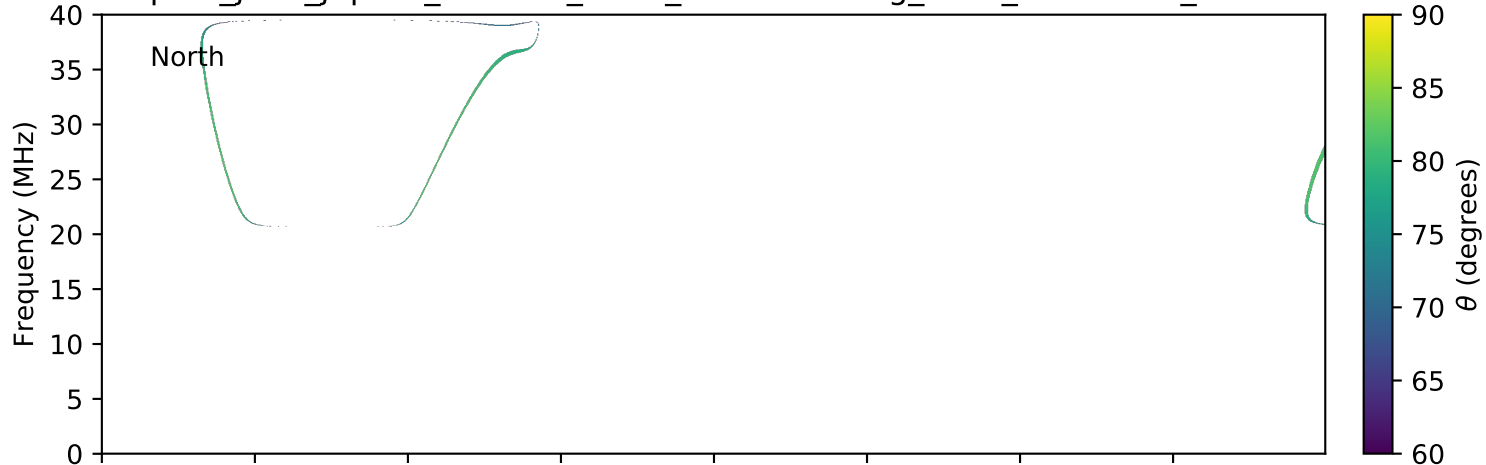
expres_juno_jupiter_215d-0r_isaac_lossc-wid1deg_5kev_20170327_v01.cdf
