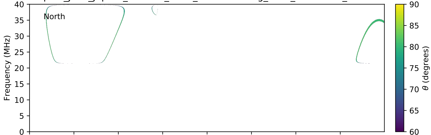
expres_juno_jupiter_171d-0r_isaac_lossc-wid1deg_5kev_20170327_v01.cdf
