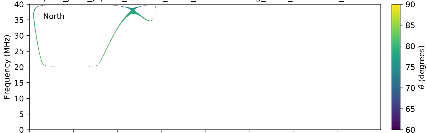
expres_juno_jupiter_146d-0r_isaac_lossc-wid1deg_5kev_20170327_v01.cdf
