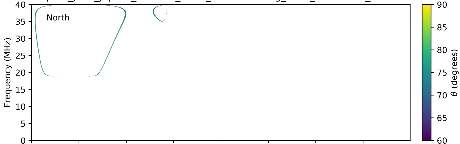
expres_juno_jupiter_134d-0r_isaac_lossc-wid1deg_9kev_20170327_v01.cdf
