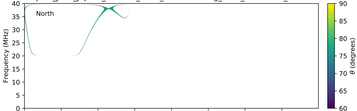
expres_juno_jupiter_134d-0r_isaac_lossc-wid1deg_5kev_20170327_v01.cdf
