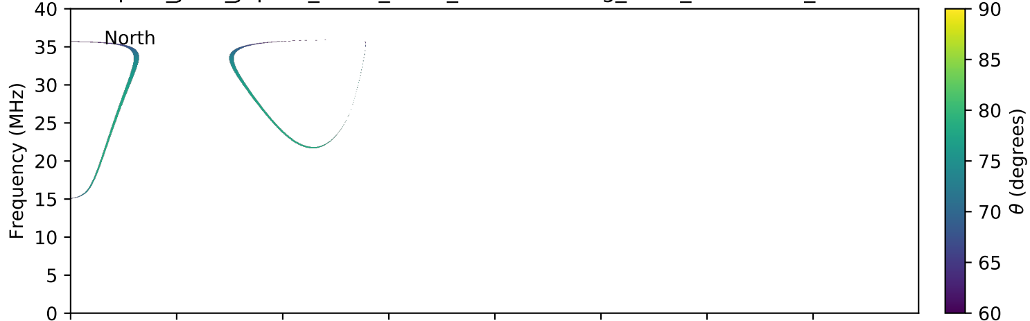
expres_juno_jupiter_0d-0r_isaac_lossc-wid1deg_9kev_20170327_v01.cdf
