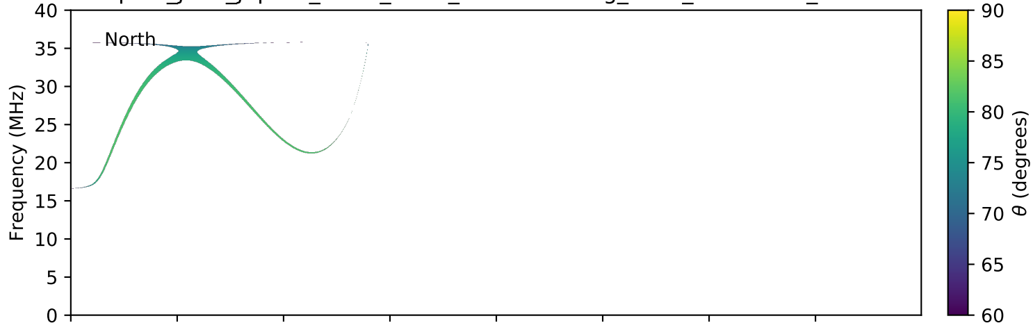
expres_juno_jupiter_0d-0r_isaac_lossc-wid1deg_5kev_20170327_v01.cdf
