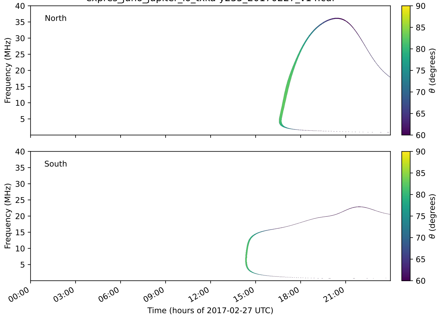
expres_juno_jupiter_io_txka-y235_20170227_v14.cdf
