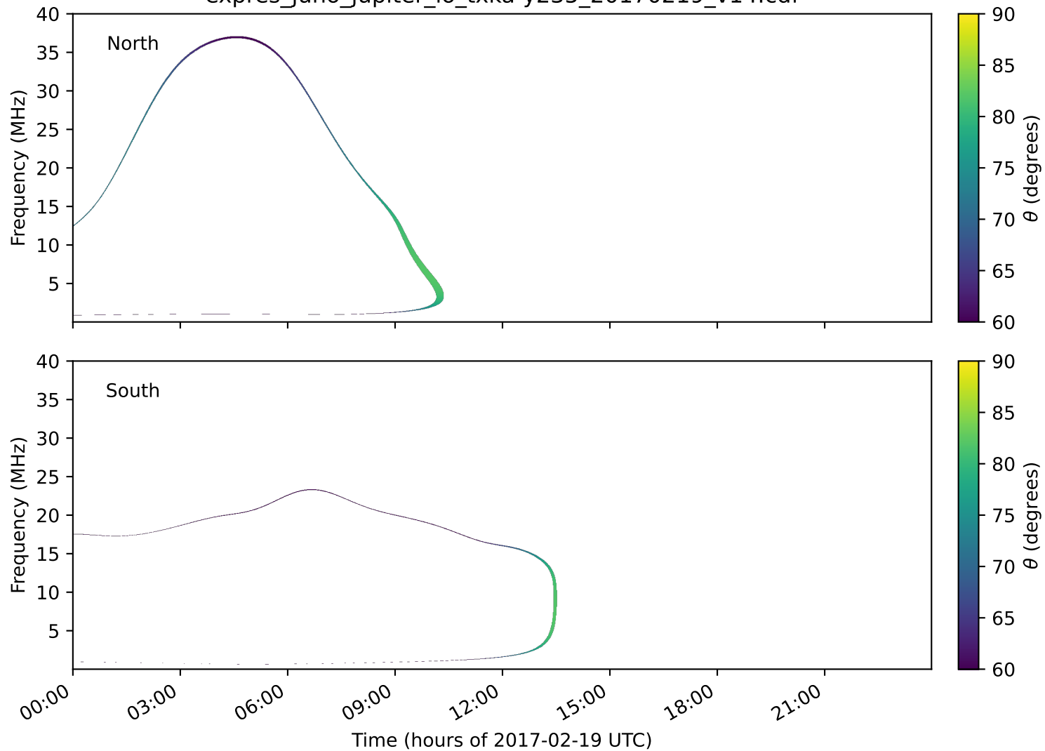
expres_juno_jupiter_io_txka-y235_20170219_v14.cdf
