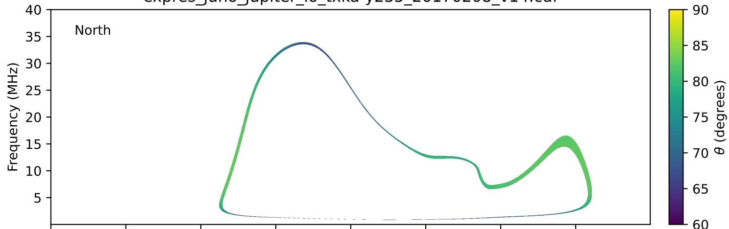
expres_juno_jupiter_io_txka-y235_20170208_v14.cdf
