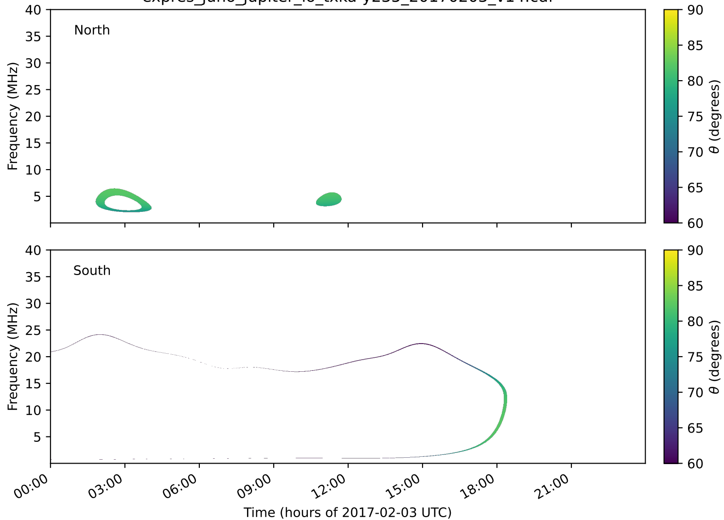
expres_juno_jupiter_io_txka-y235_20170203_v14.cdf
