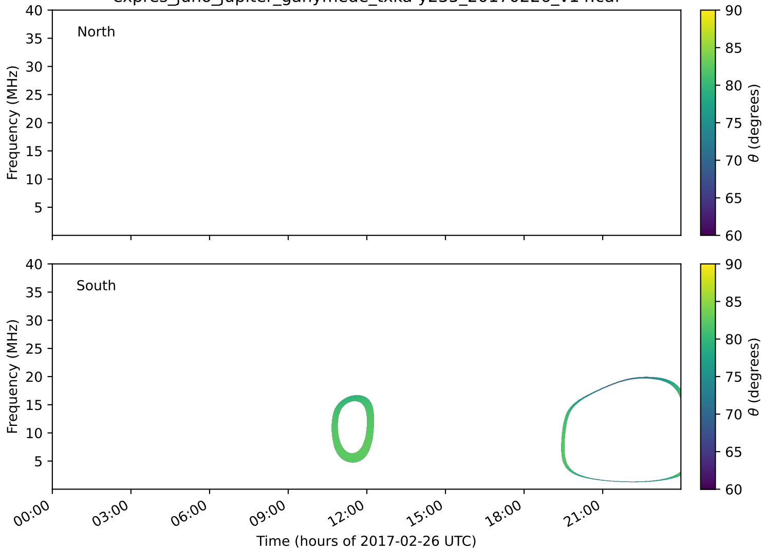
expres_juno_jupiter_ganymede_txka-y235_20170226_v14.cdf
