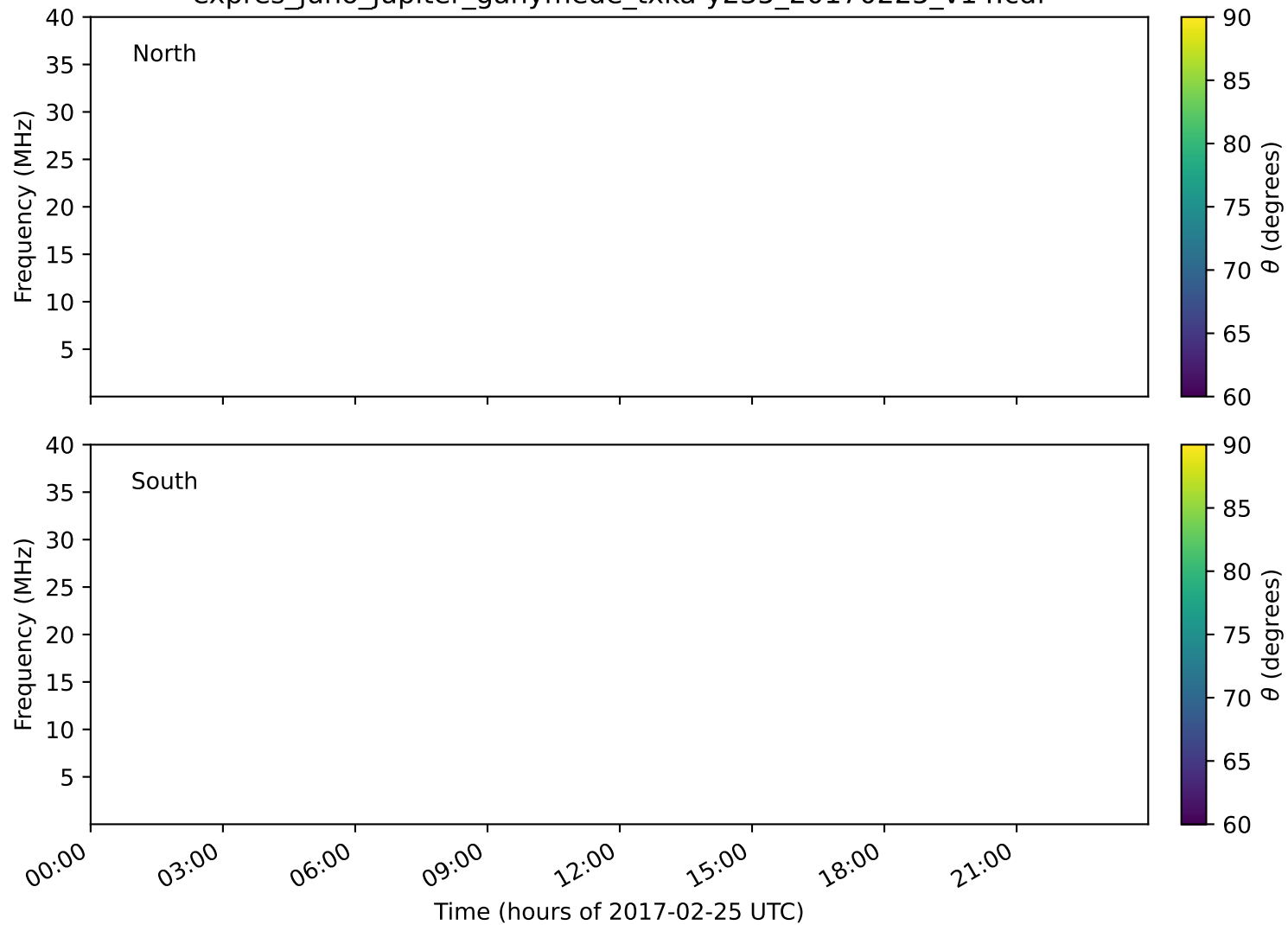
expres_juno_jupiter_ganymede_txka-y235_20170225_v14.cdf
