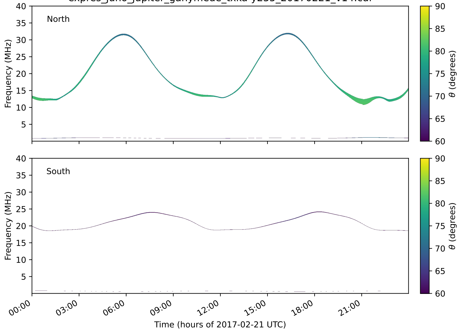
expres_juno_jupiter_ganymede_txka-y235_20170221_v14.cdf
