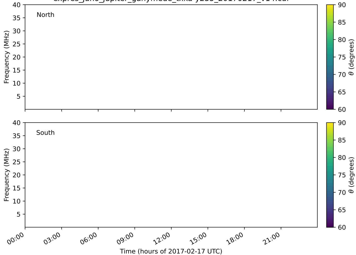
expres_juno_jupiter_ganymede_txka-y235_20170217_v14.cdf
