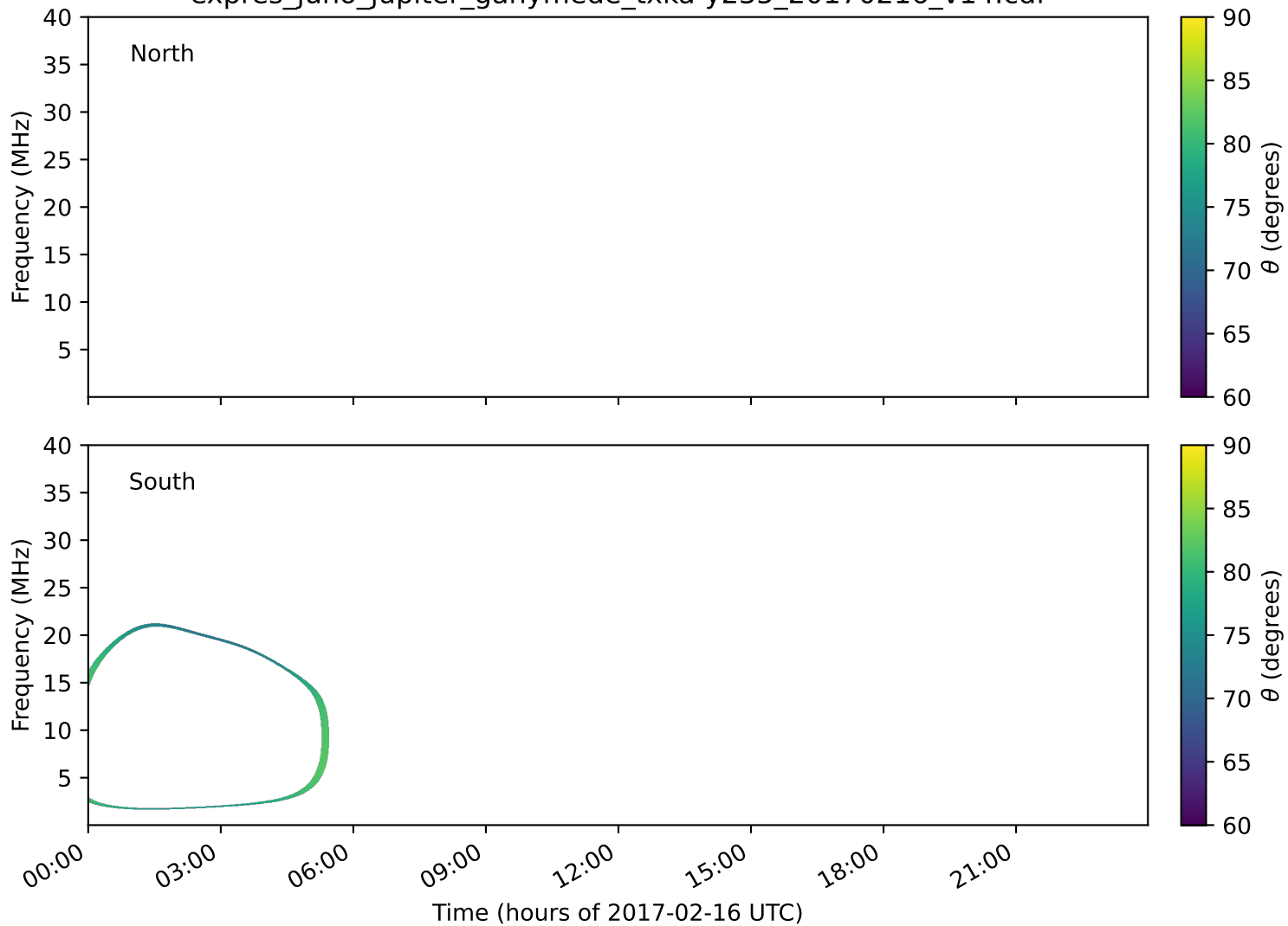
expres_juno_jupiter_ganymede_txka-y235_20170216_v14.cdf
